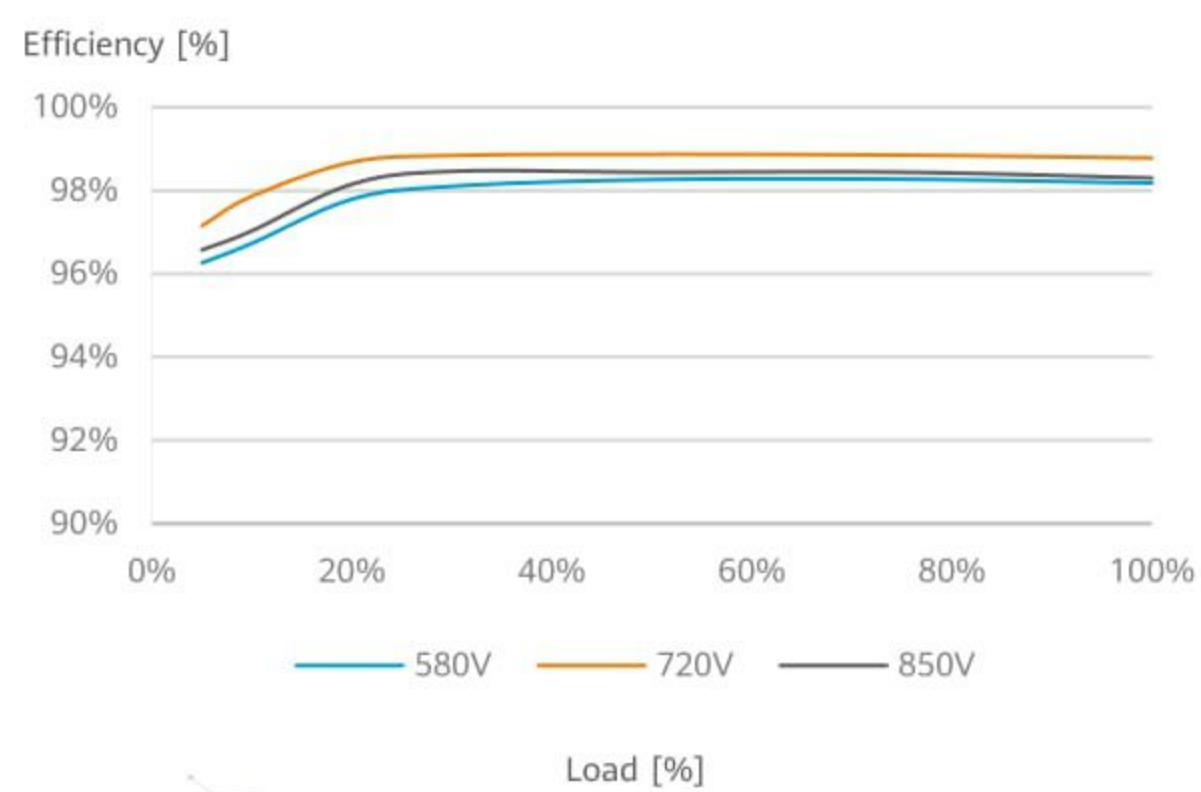
Efficiency Curve
