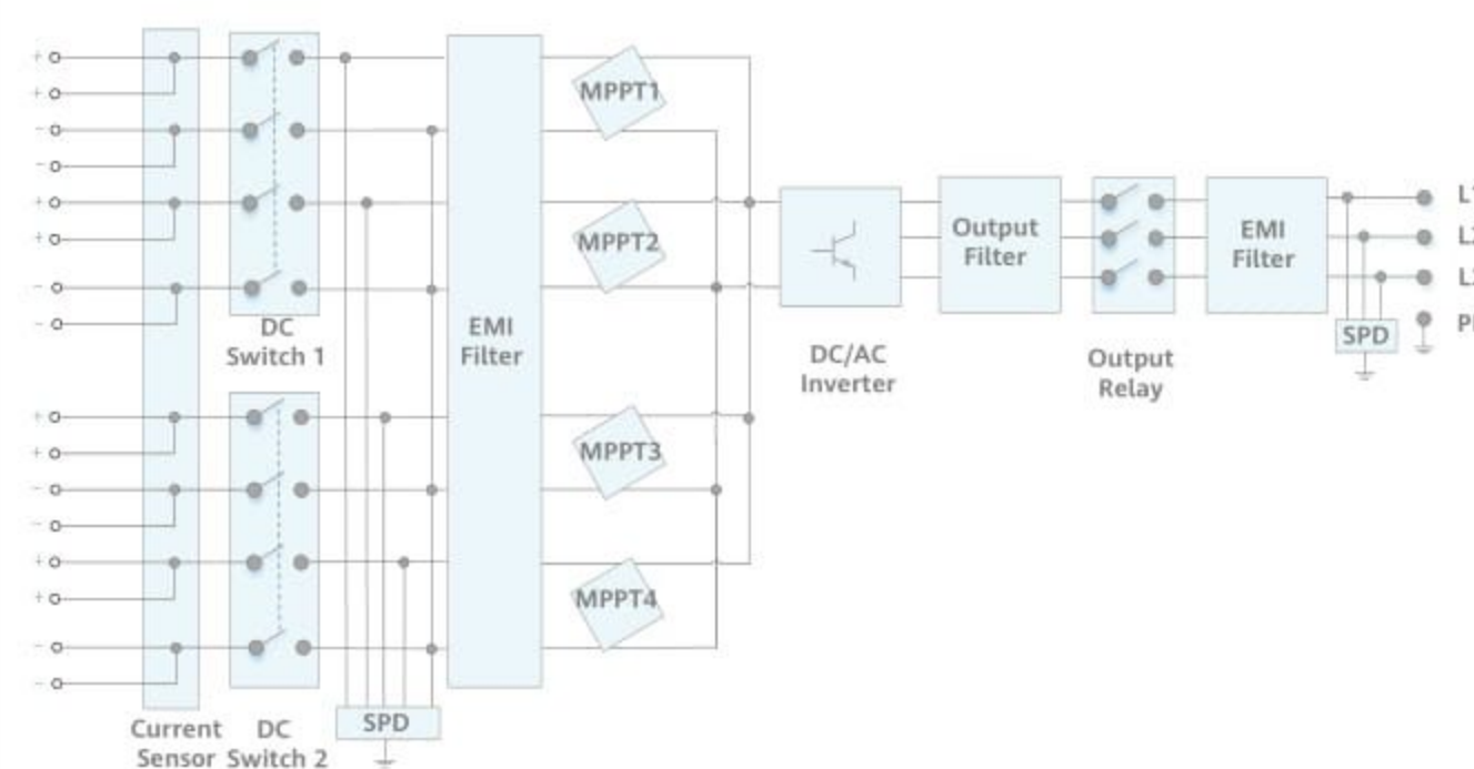
Circuit Diagram
